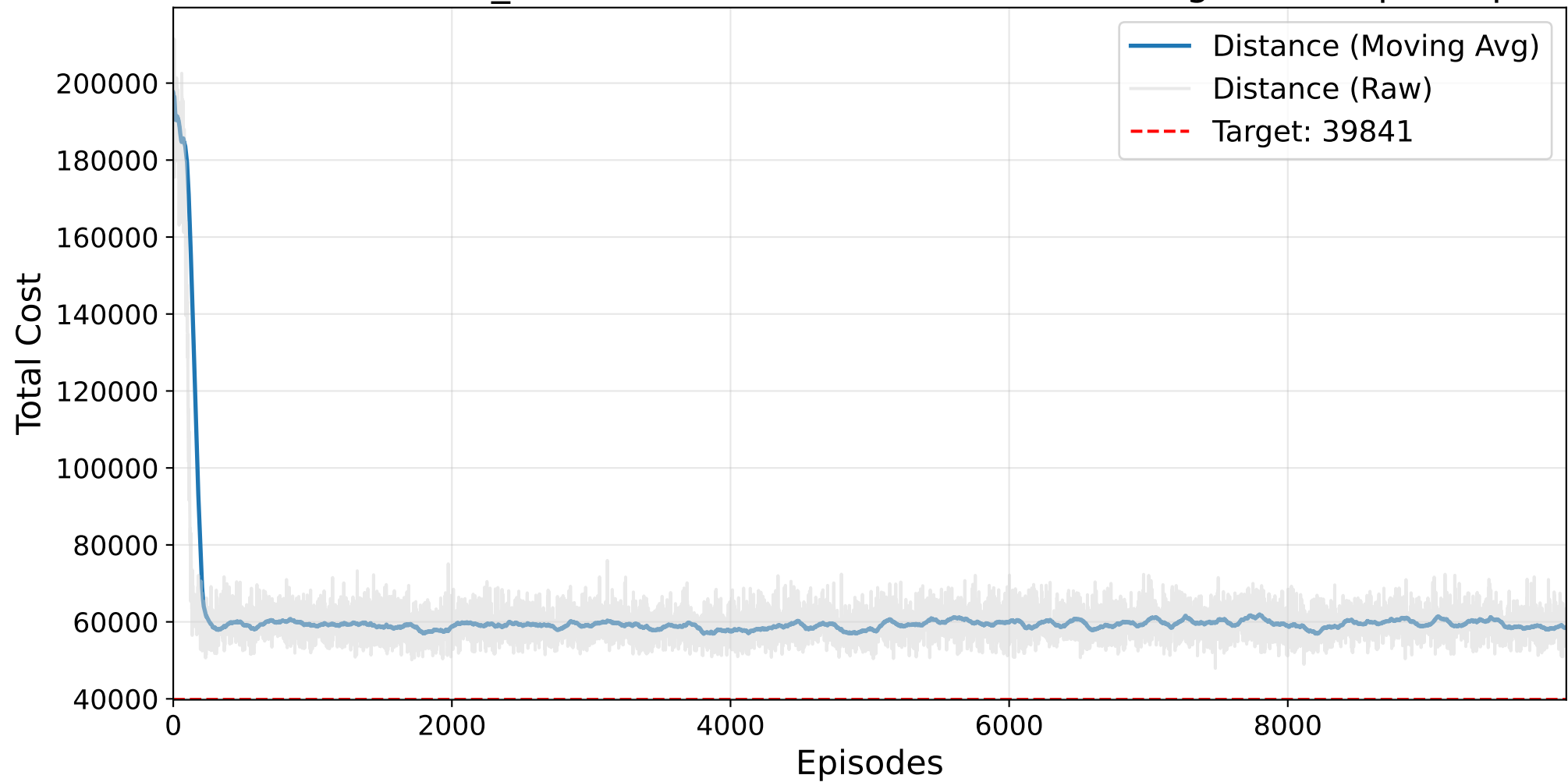
Final RANDOM_SEARCH Masked AutoRL-SOP Training - kro124p.2.sop
